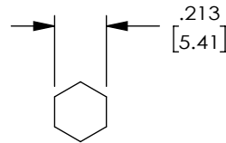
RECOMMENDED FERRULE CRIMP SIZE
