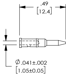
CONTACT (SOLDER OR CRIMP .068" [1.72])
