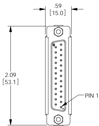
DB25 FEMALE CONNECTOR
