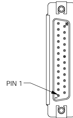
DB25 MALE CONNECTOR
