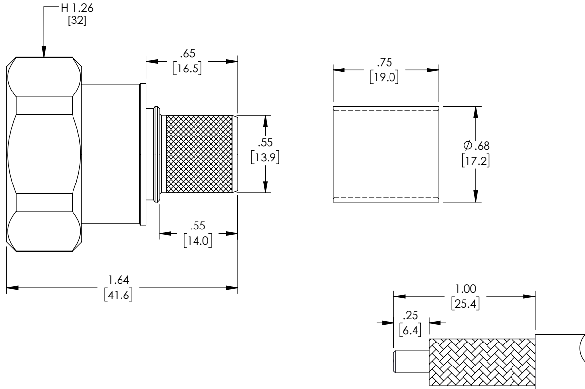
RECOMMENDED CABLE STRIPPING DIMENSIONS
