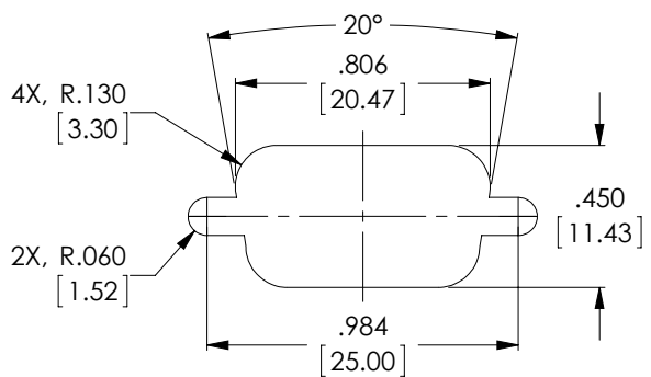
RECOMMENDED PANEL OPENING
