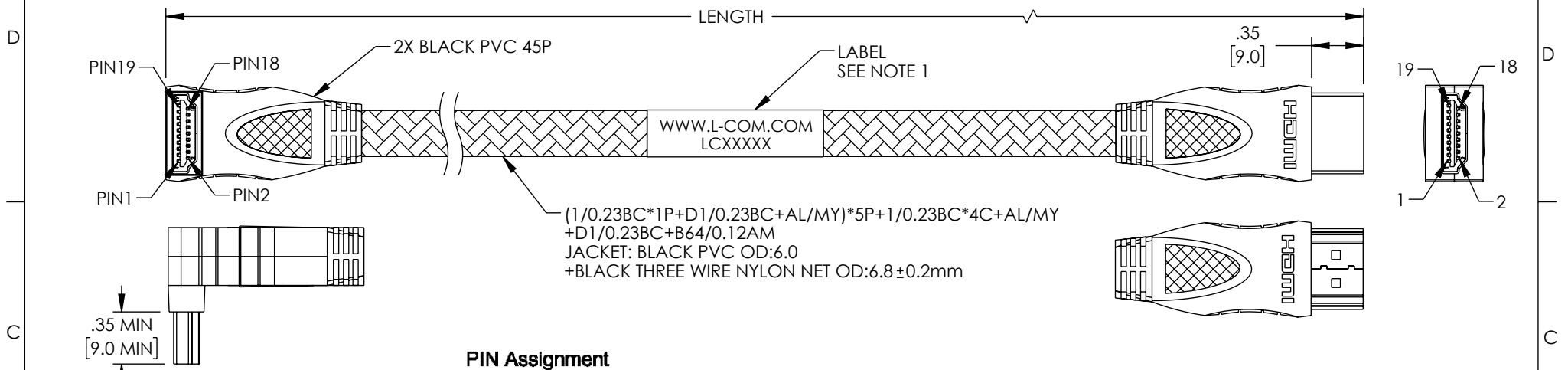
P2 HDMI FM 19P PIN:G/F, SHELL: GOLD PLATED
