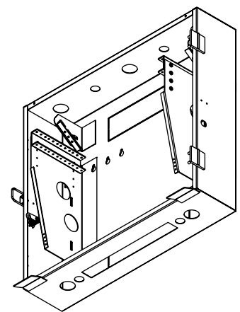
VIEW A-A POPULATED ENCLOSURE DOOR NOT SHOWN
