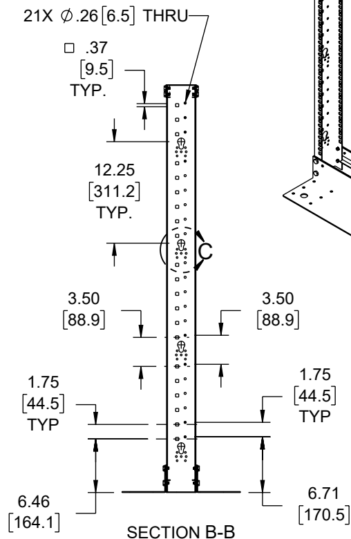
SECTION B-B
