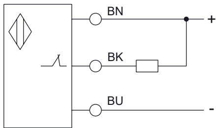
NPN NC CONNECTION DIAGRAM
