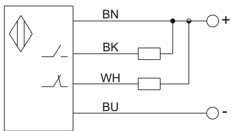
NPN NO+NC CONNECTION DIAGRAM
