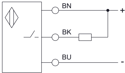
NPN NO CONNECTION DIAGRAM
