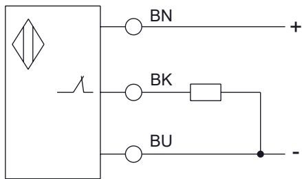
PNP NC CONNECTION DIAGRAM
