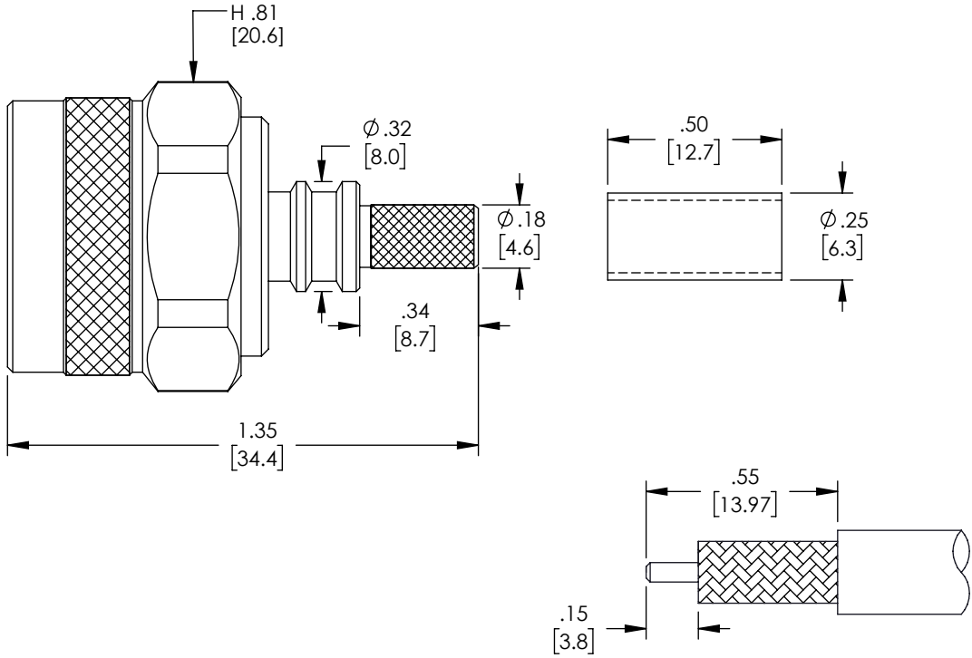
RECOMMENDED CABLE STRIPPING DIMENSIONS
