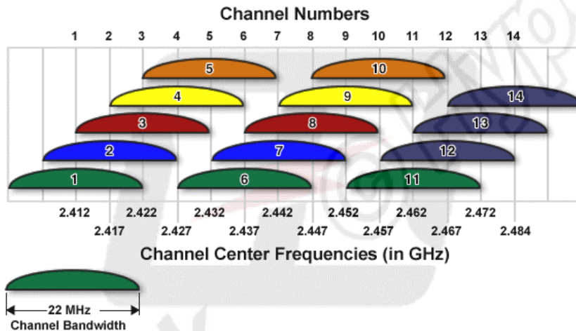
IEEE 802.11 RF Channelization Scheme
