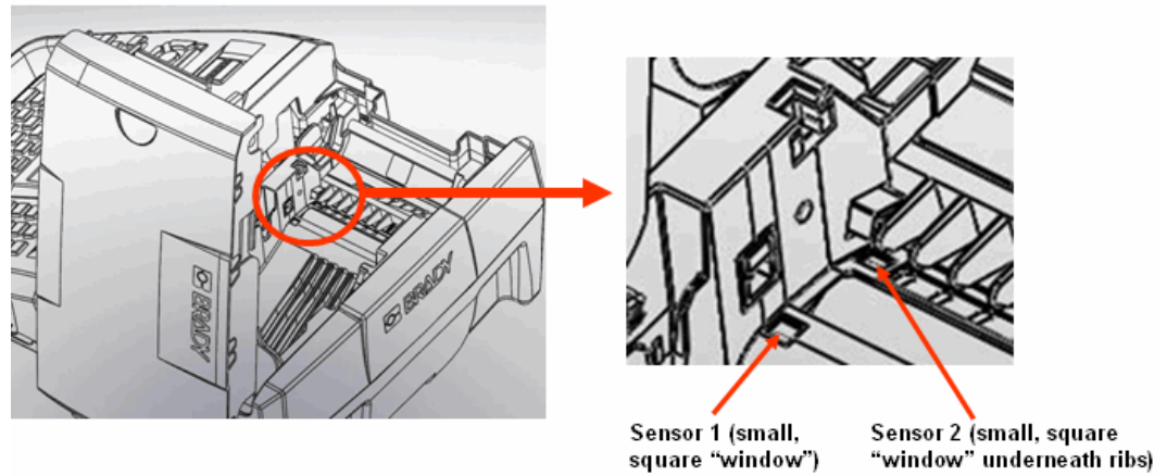
Figure 14 • Sensor locations
