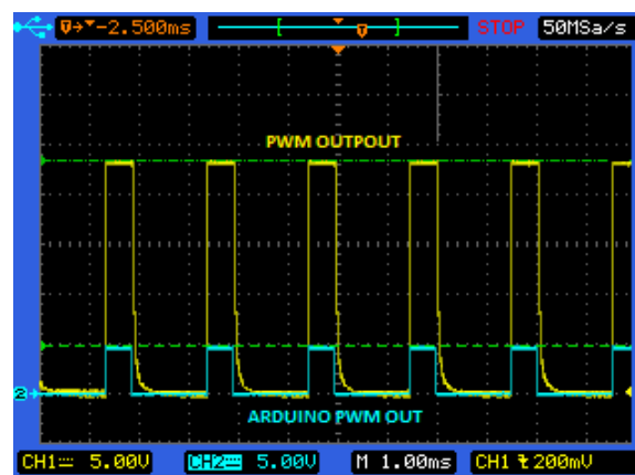
PWM Waveform:
