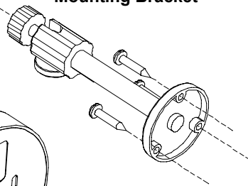
HGX-PMT02 - Small Metal Tilt-and-Swivel Wall Mounting Bracket
