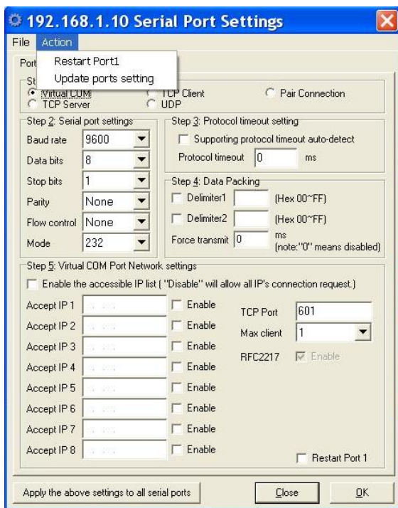
Fig 75. Action
