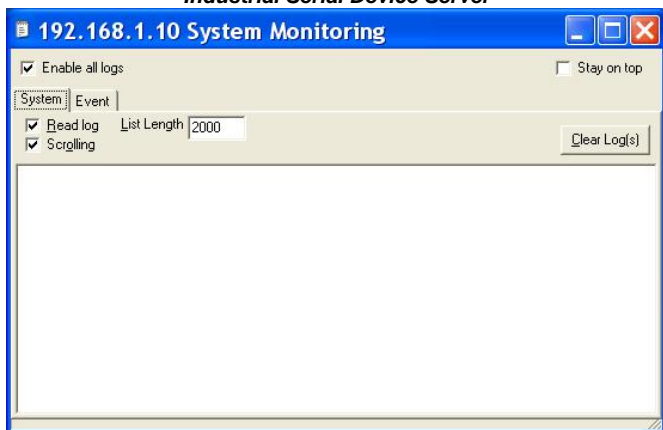
Fig 87. System
