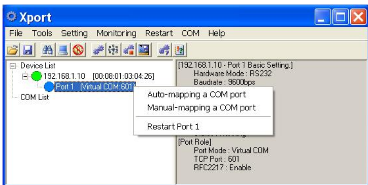
Fig 52. Serial port
