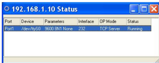
Fig 86. Port Status
