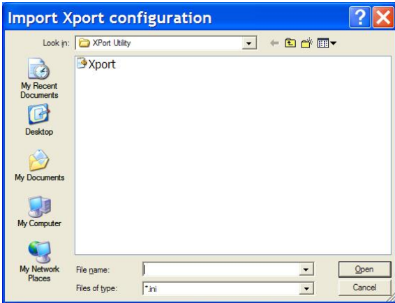
Fig 72. Import Configuration
