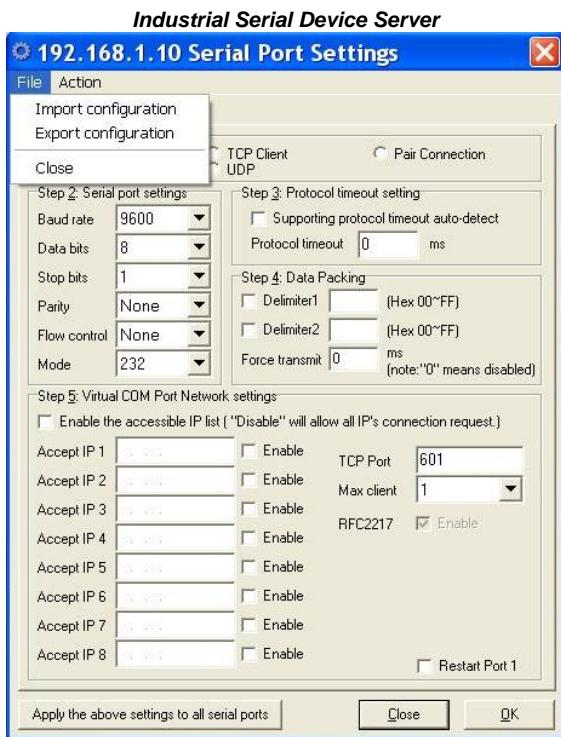
Fig 71. File
