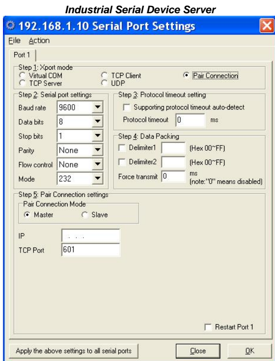
Fig 80. Pair Connection
