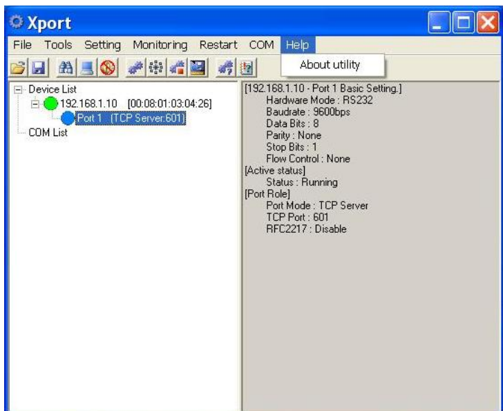
Fig 96. Help
