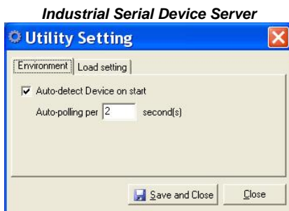
Fig 83. Environment
