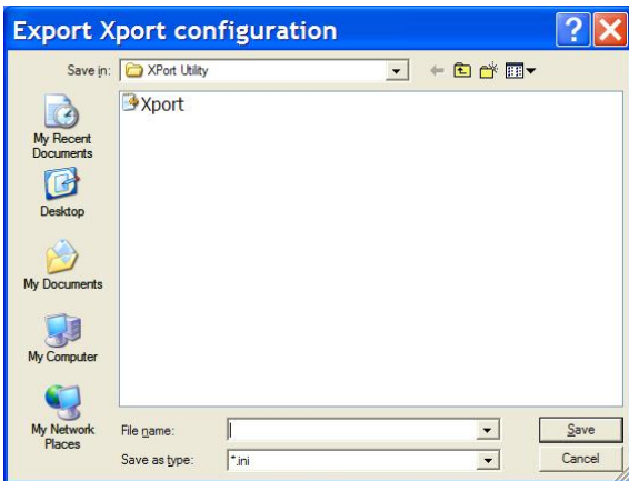
Fig 73. Export Configuration
