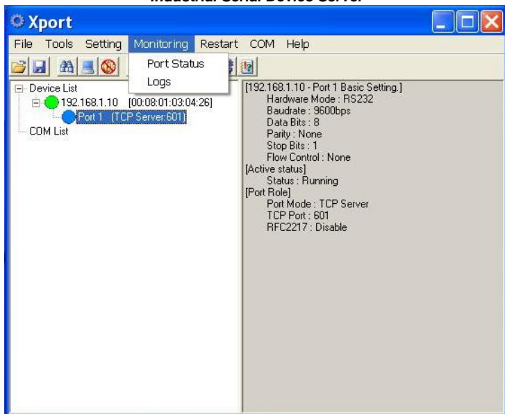
Fig 85. Monitoring
