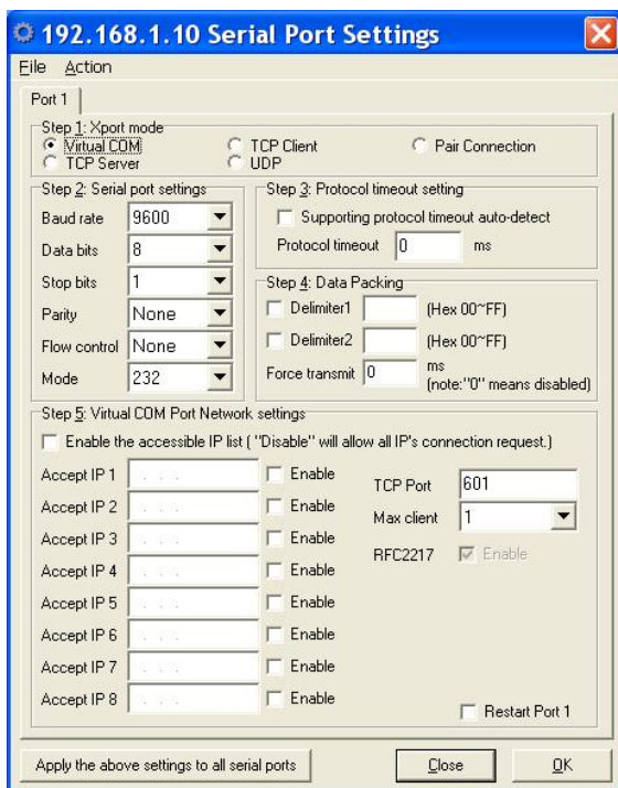
Fig 76. Virtual COM
