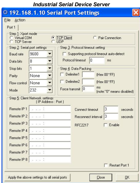
Fig 78. TCP Client
