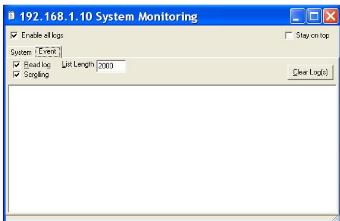
Fig 88. Event
