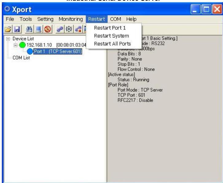
Fig 89. Monitoring
