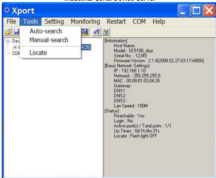
Fig 67. Tools
