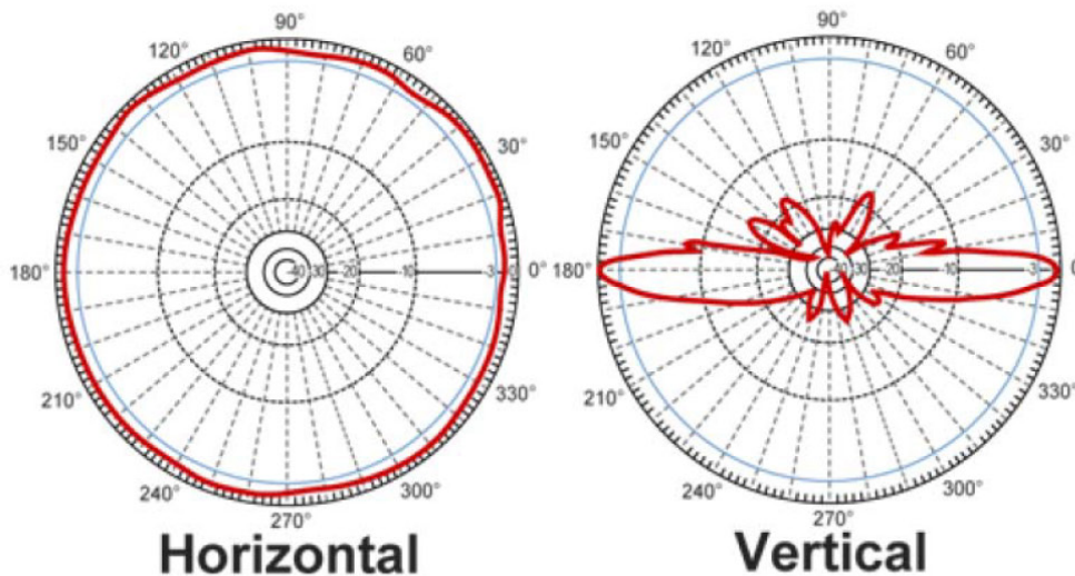
Typical Omni directional antenna radiation pattern (HG2415U-PRO)
