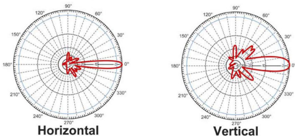
Typical Directional Antenna Radiation Pattern (HG2424EG-NF)
